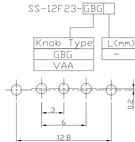
P.C.B LAYOUT BOTTOM VIEW
