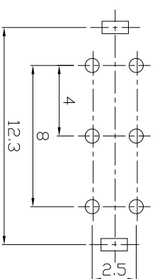
P.C.B LAYOUT BOTTOM VIEW
