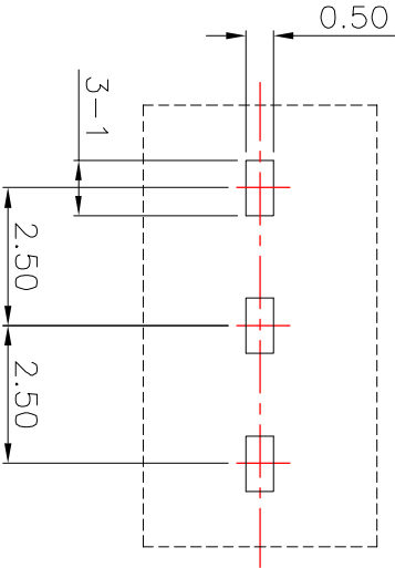
Hole Layout(top view)
