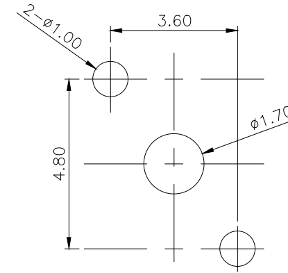
PCB LAND DIMENSION
