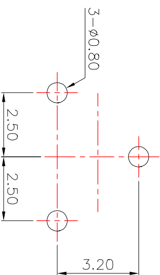
HOLE LAYOUT
