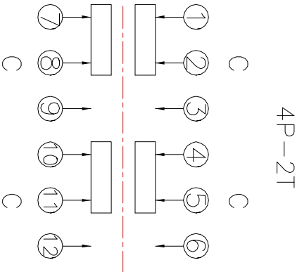
Circuit Diagram
