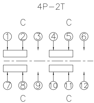
Circuit Diagram
