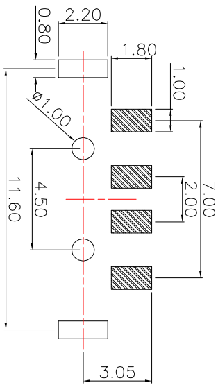
PCB Layout
