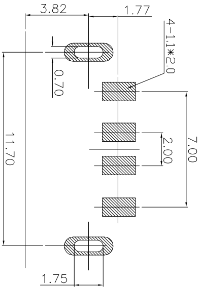
PCB Layout
