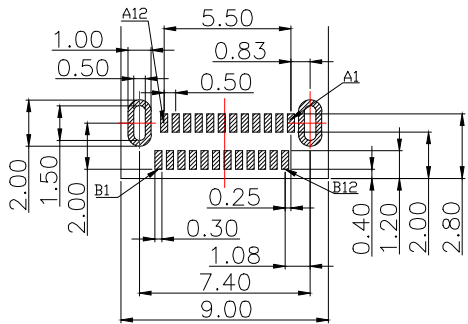
RECOMMENDED P.C.B. LAYOUT (T:1.00mm) TOLERANCE UNSPECIFIED ±0.05mm
