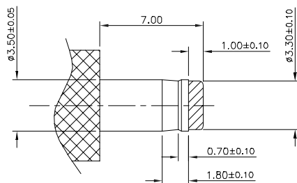
(ø3.50mm DC PLUG DETAIL DRAWING)
