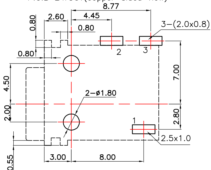
P.C.B LAYOUT(copper-sided view)
