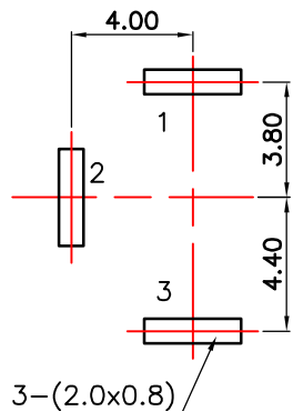
P.C.B LAYOUT(copper-sided view)
