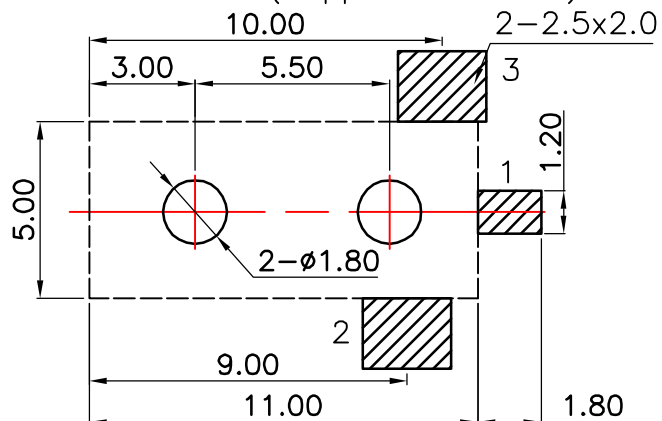
P.C.B LAYOUT(Copper-side view)
