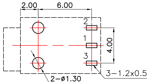
P.C.B LAYOUT(Copper-side view)
