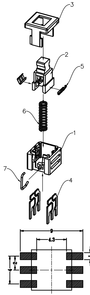
P.C.B LAYOUT BOTTOM VIEW
