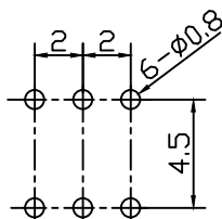
P. C. B LAYOUT
