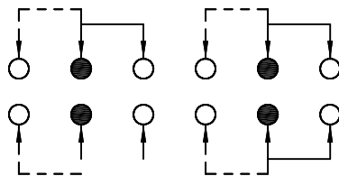
SCHEMATIC (SHORTING/NON-SHORTING)
