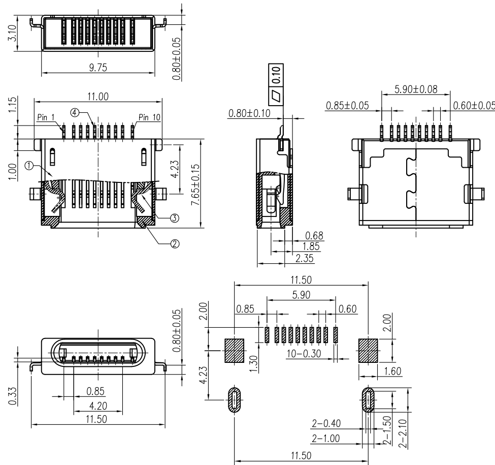
RECOMMENDED P.C.B HOLE LAYOUT COMPONENT SIDE VIEW(TOLERANCE: +/-0.05)
