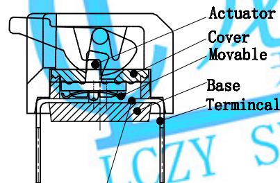
Terminal contact
