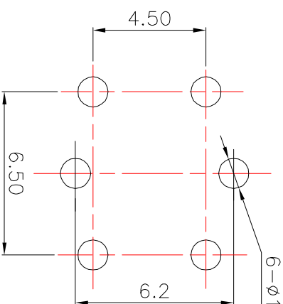
PCBLayout(Pattern Side)
