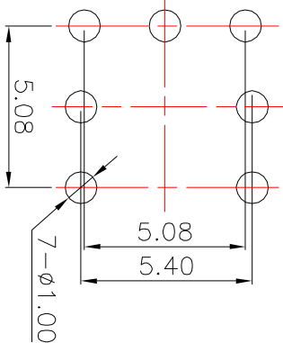
PCBLayout(Pattern Side)
