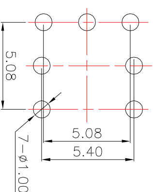
PCBLayout(Pattern Side)
