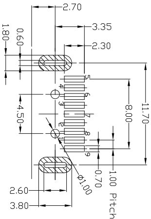
RECOMMEND PCB LAYOUT (TOLERANCE:±0.05)
