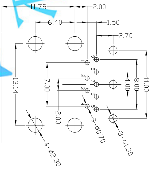
RECOMMEND PCB LAYOUT
