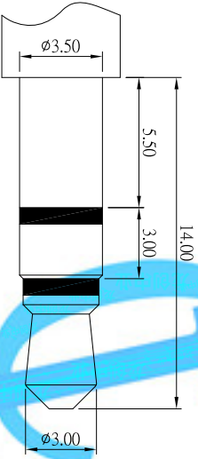
Ø3.50mm 3 POLE PLUG
