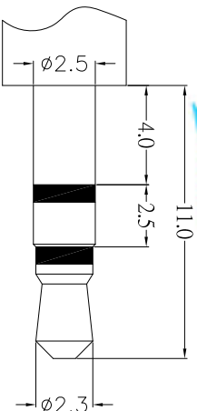
Ø2.50mm 3 POLE PLUG
