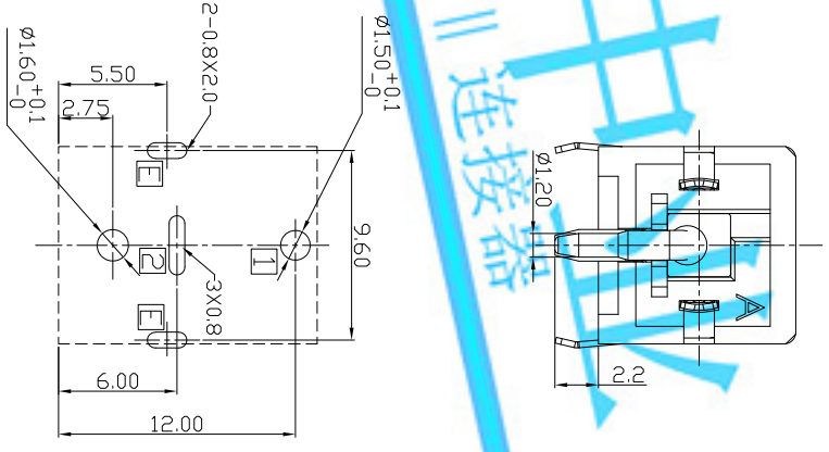
RECOMMENDED P.C.B. LAYOUT UNSPECIFIED TOLERANCE: \pm 0.05 (TOP VIEW)
