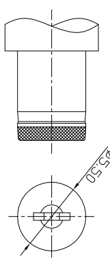
DC MATE PLUG
