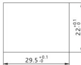
安装孔尺寸 MOUNTING HOLE DIMENTION
