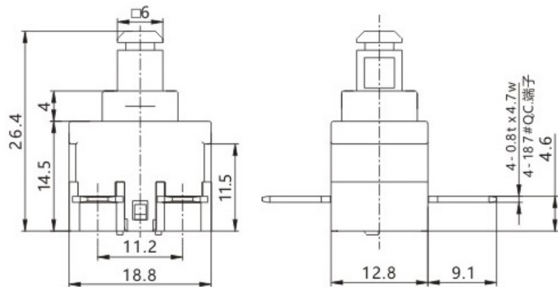
安装孔尺寸 MOUNTING HOLE DIMENTION
