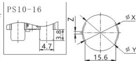
安装孔尺寸 MOUNTING HOLE DIMENTION
