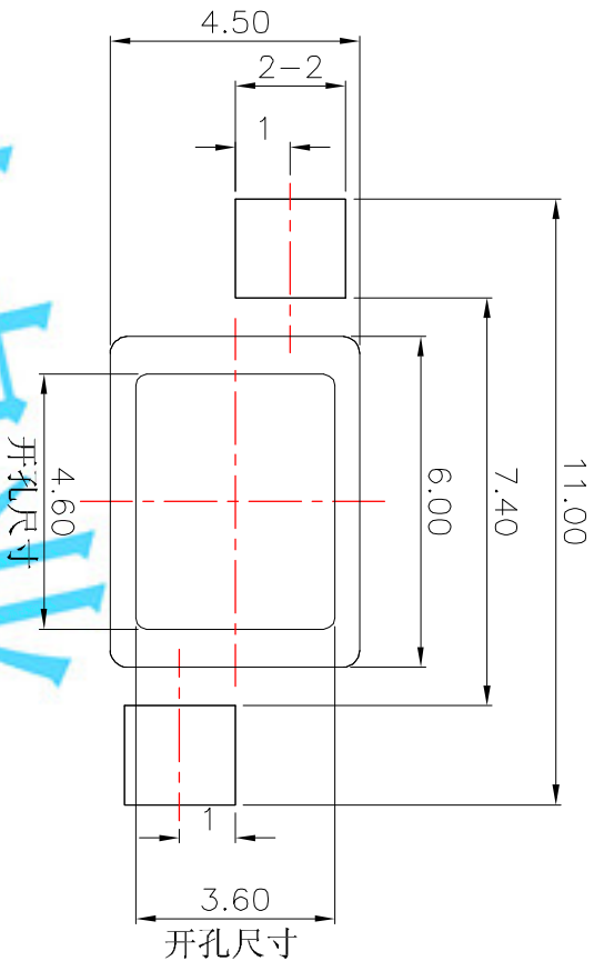
Hole Layout(top view)
