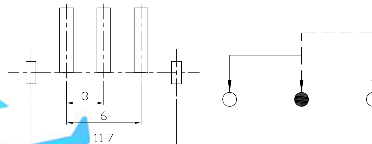
P.C.B LAYOUT BOTTOM VIEW
