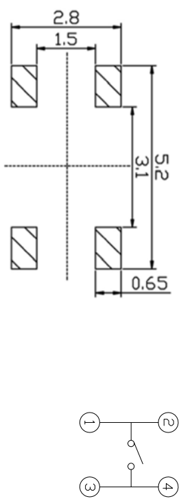
P.C.B MOUNTING PATTERN DIMENSION CIRCUIT DIAGRAM The following soldering patterns are recommended for reflow soldering
