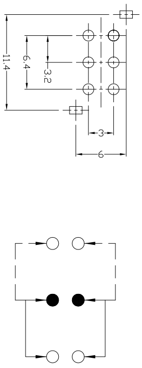
P.C.B LAYOUT BOTTOM VIEW
